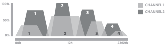
Fig. 3 - Operating time diagram
